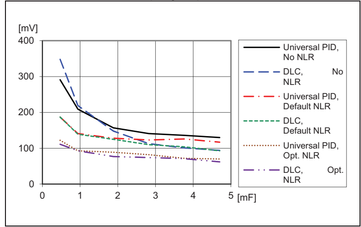
Load transient peak voltage deviation vs. decoupling capacitance. Step (6.25-18.75-6.25 A). Parallel coupling of capacitors with 470\text{ }\mu\text{F}/10\text{ m}\Omega , T_{P1} = +25^\circ\text{C} , V_I = 12\text{ V} , V_O = 3.3\text{ V} , f_{sw} = 320\text{ kHz} , di/dt = 2\text{ A}/\mu\text{s}
