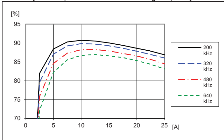
Efficiency vs. load current and switching frequency at T_{P1} = +25^\circ\text{C} , V_I = 12\text{ V} , V_O = 1.0\text{ V} , C_O = 470\text{ }\mu\text{F}/10\text{ m}\Omega . Default configuration except changed frequency
